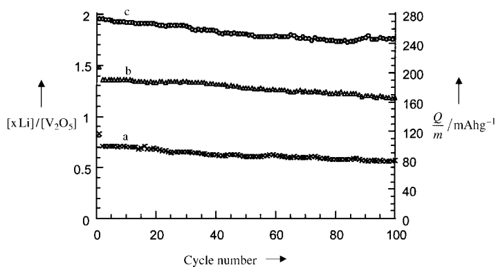
Figure 5. Capacity retention on cycling for a) V_2O_5 xerogel, b) V_2O_5/C , and c) V_2O_5/C -PEG. Current density: 100 mA\ g^{-1} ; potential range: 3.8–1.8 V.
