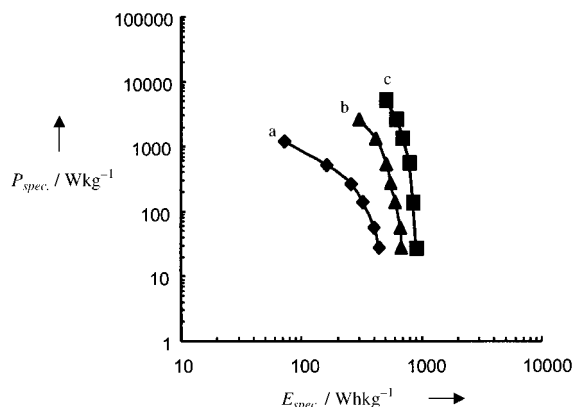
Figure 4. Power ( P )–energy ( E ) plots of a) V_2O_5 xerogel, b) V_2O_5/C , and c) V_2O_5/C -PEG that illustrate the rate response.
